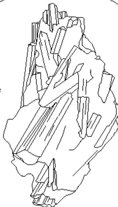
Kyanite
