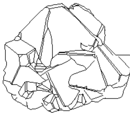
Pyrite
