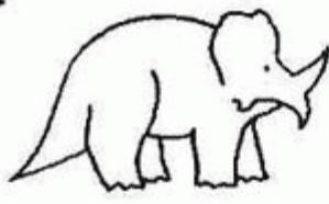
Monoclonius
